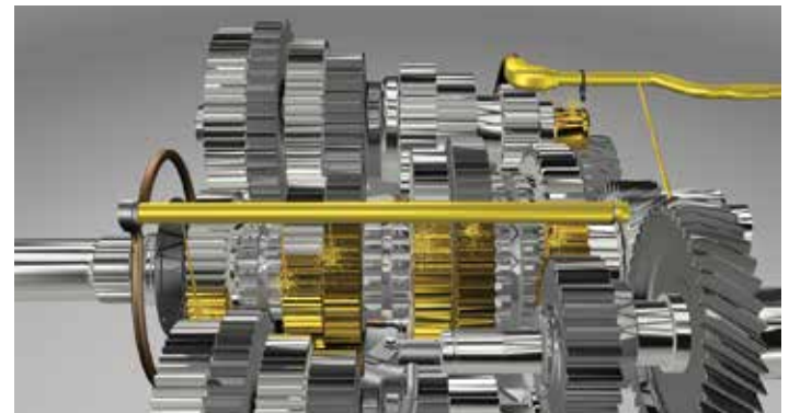
Precision lube system eliminates oil cooler and reduces remaining transmission inefficiencies by nearly one-third.
